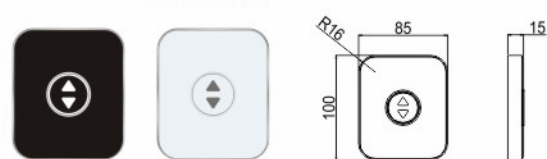
GH-GS02C-別墅梯外呼
