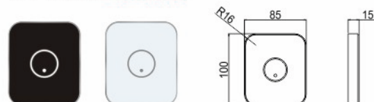
GH-GS03C-別墅梯外呼
