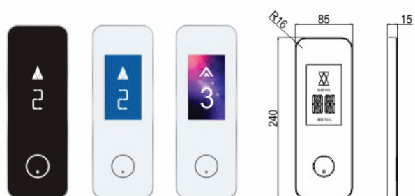
GH-GS02C-別墅梯外呼
